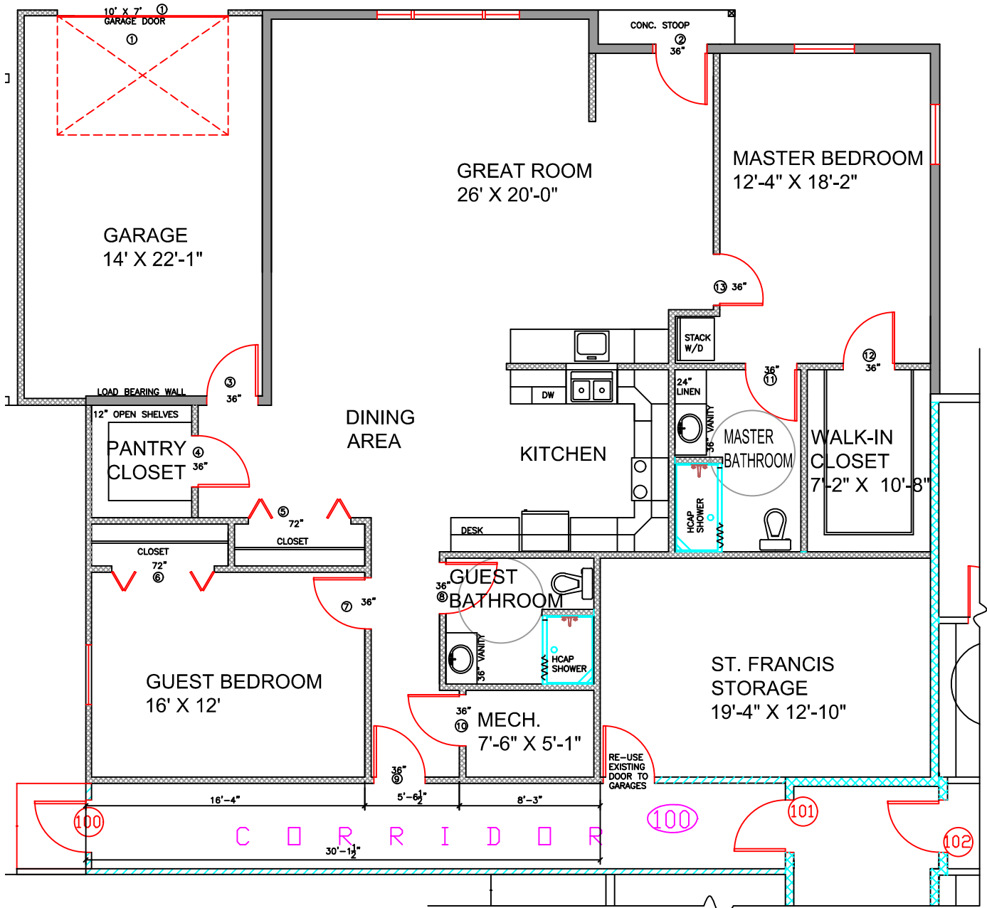
NED POSTEL'S APARTMENT SCALE: 1/8" = 1'
